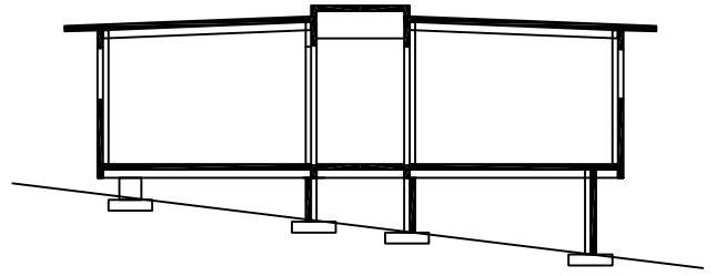
SLOPING SITE FOOTINGS & PRECAST FOUNDATION WALLS
